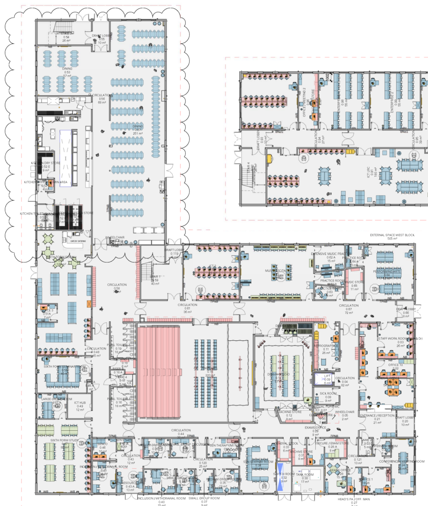
Ground Floor - Block B
